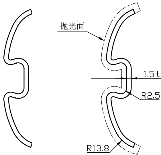
Section A-A (2:1)
